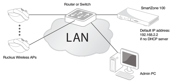
FIGURE 4 Connecting the admin PC, SZ300, and Ruckus Wireless APs to the network
